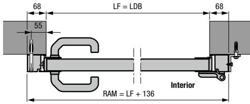
Side door with aluminium block frame, profile type 2 Fitting behind the opening
