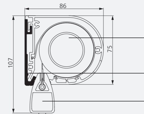
Cassette round, small (86 x 75 mm)
