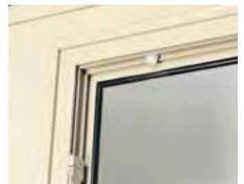
The electromagnetic safety sensor is installed in power-operated doors.
