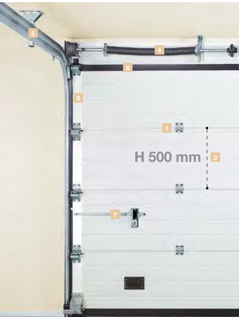
Internal view of a typical sectional door present on the market.
