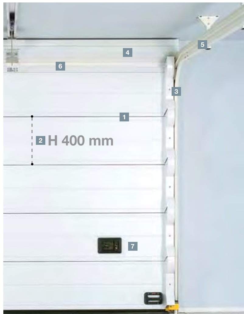
Internal view of a power-operated New Age XT sectional door.
